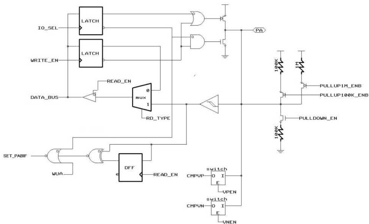
Figure 5 Block Diagram of PA0 & PA1
