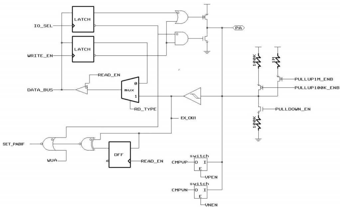
Figure 6 Block Diagram of PA2
