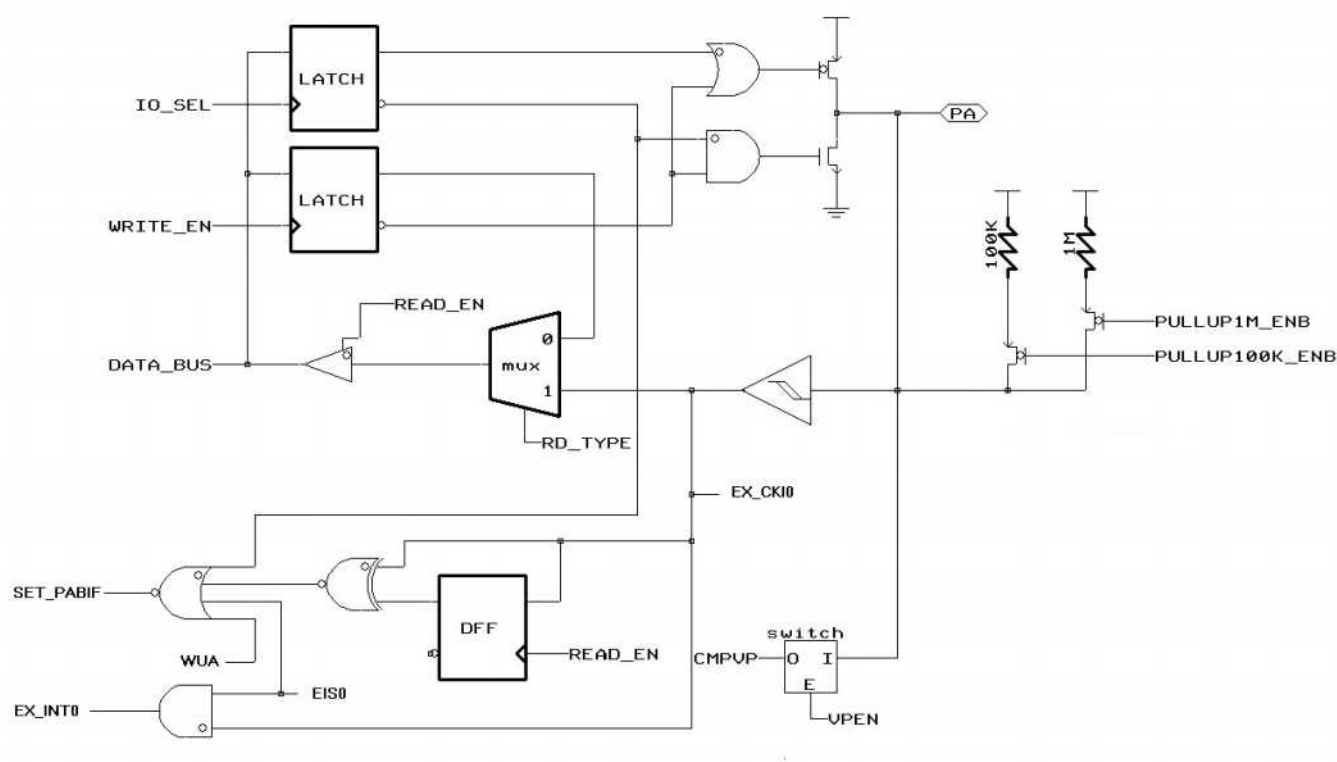
Figure 8 Block Diagram of PA4
