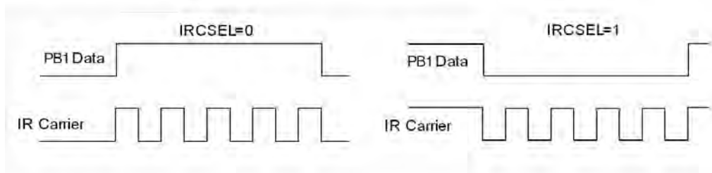
Figure 29 Polarity of IR Carrier vs. Output Data
